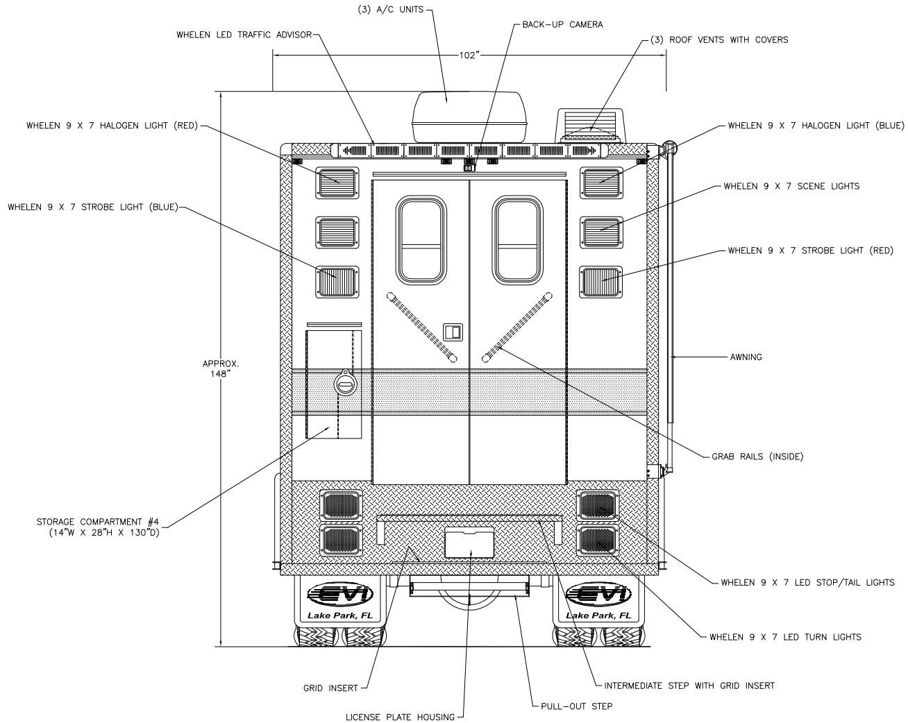
Rear View
