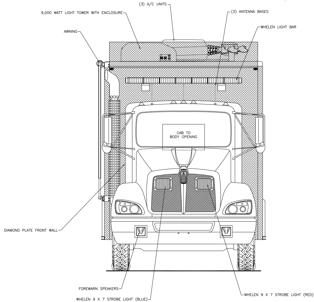
Front View
