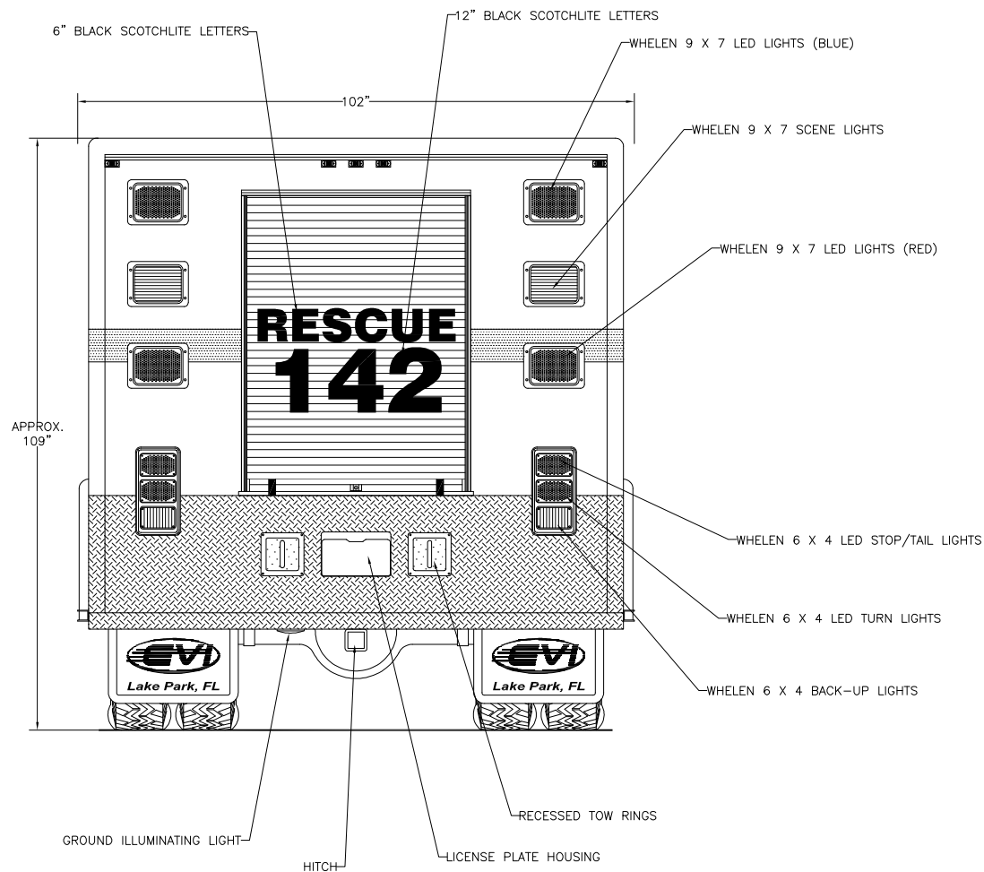
Rear View
