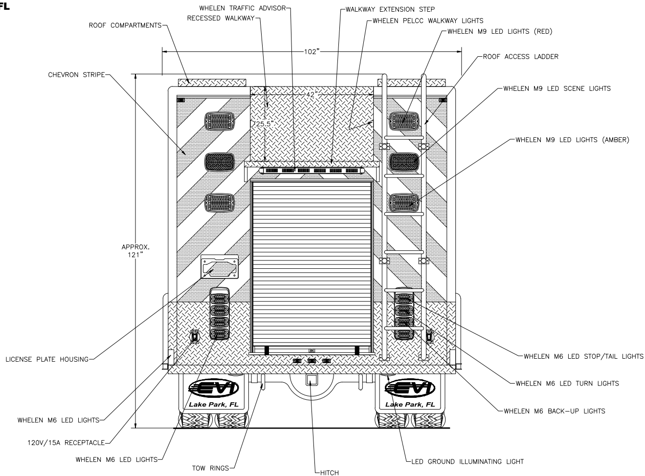
Rear View
