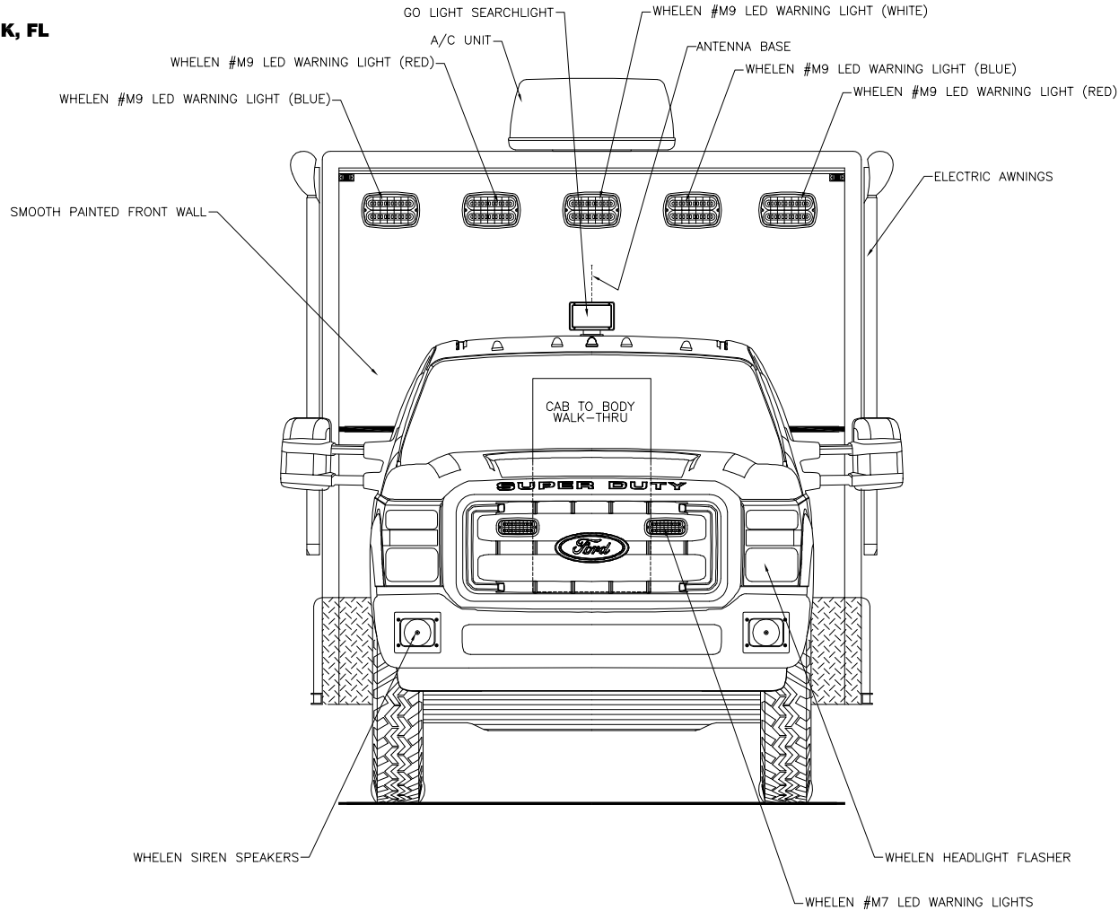
Front View
