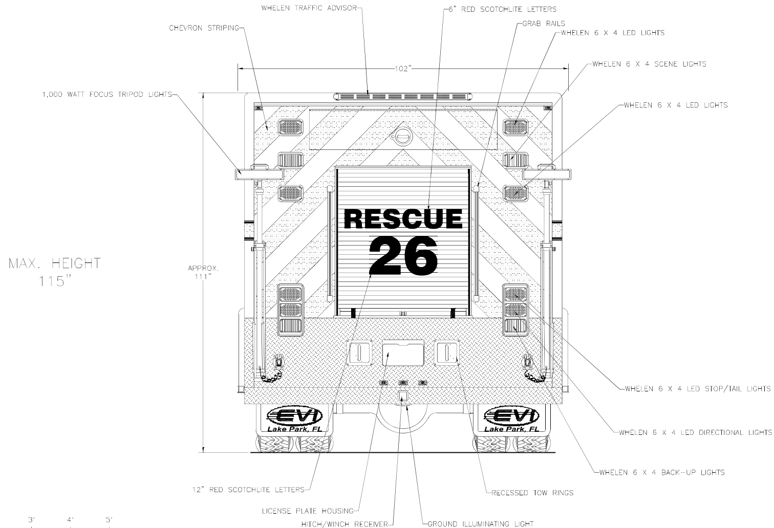
Rear View
