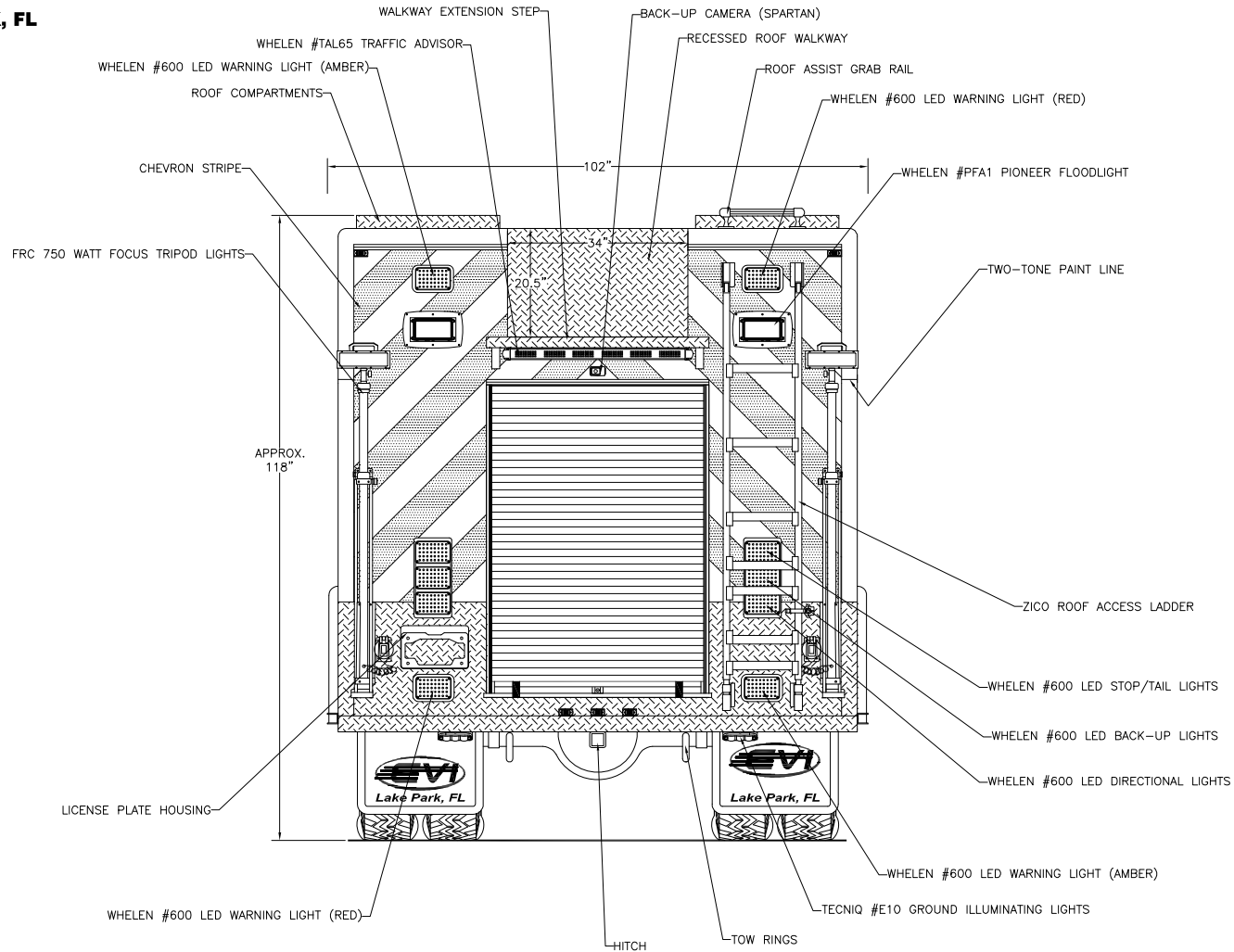
Rear View
