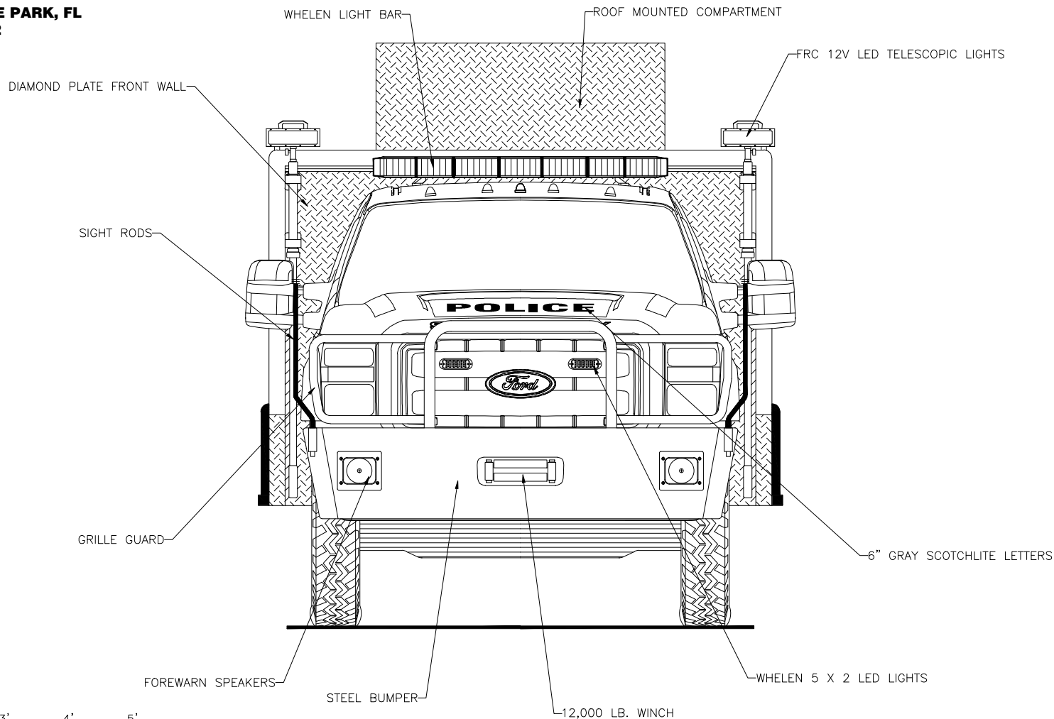
Front View
