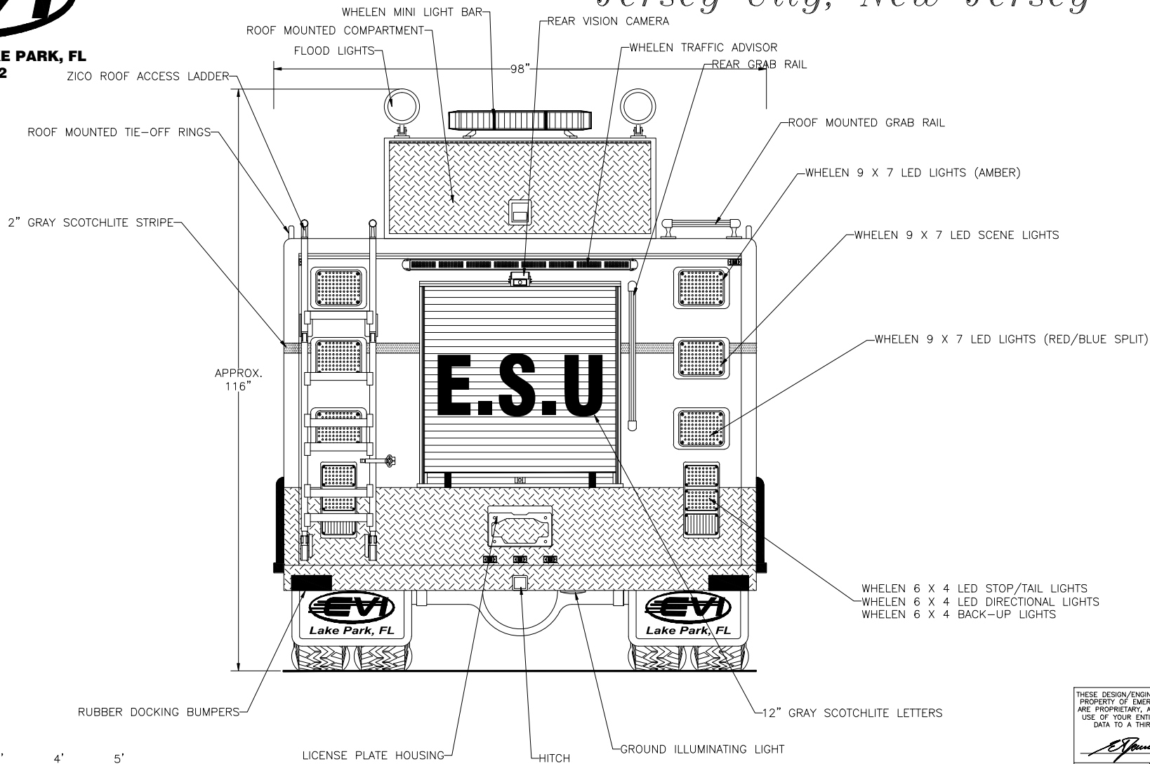
Rear View
