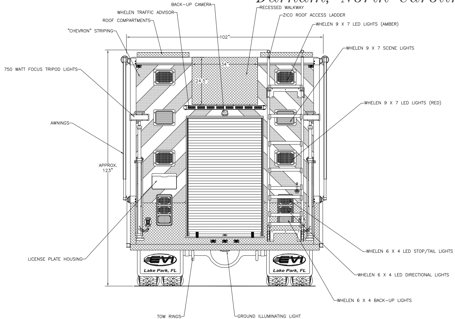
Rear View
