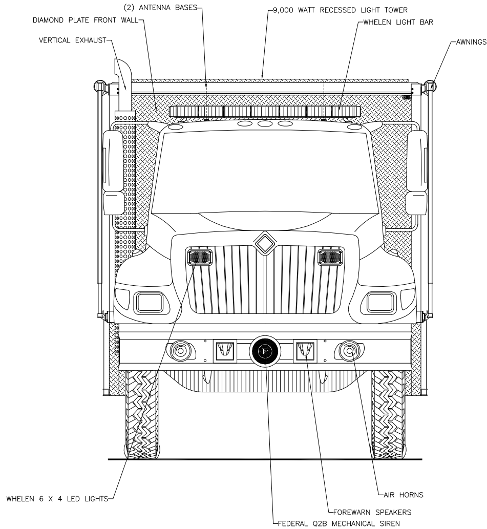
Front View
