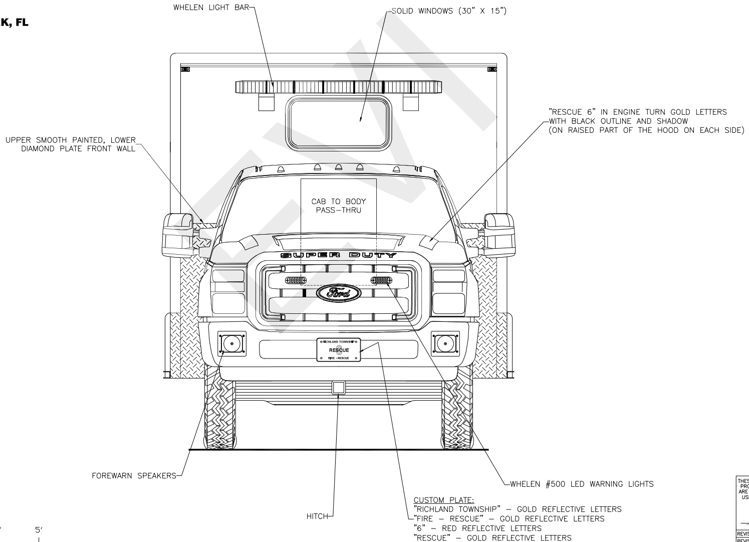
Front View
