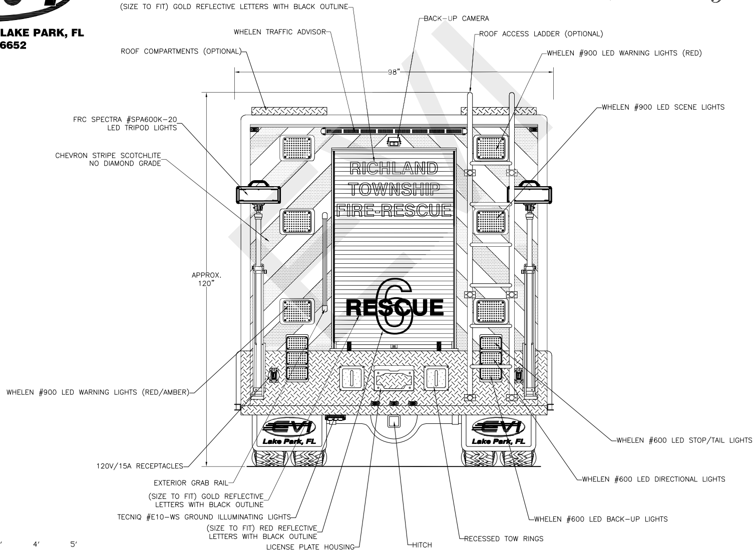
Rear View
