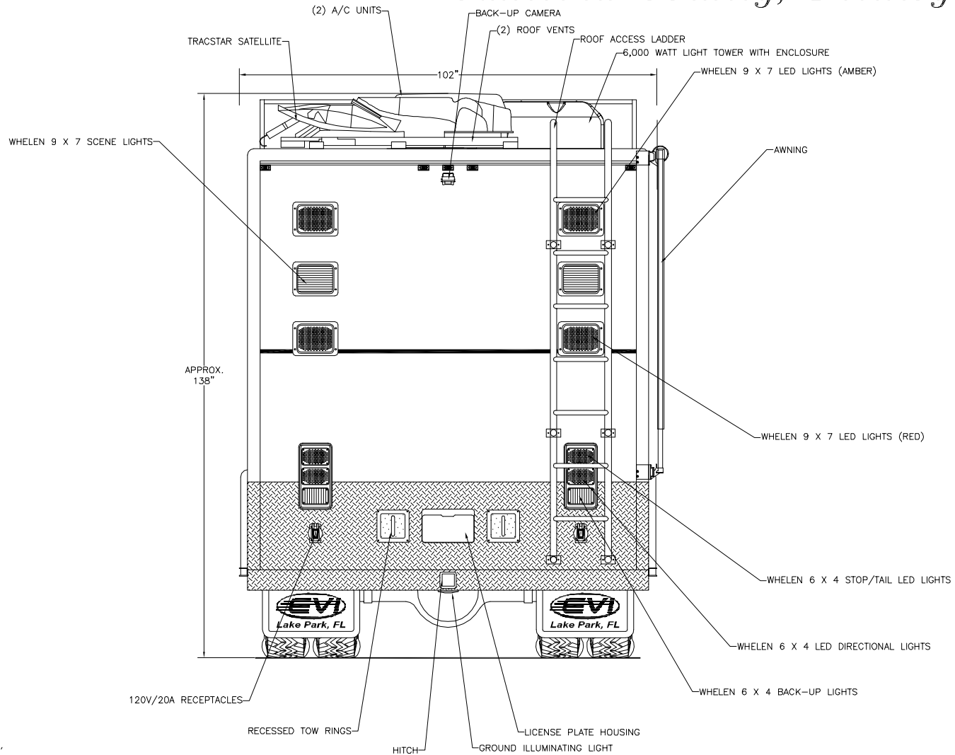
Rear View
