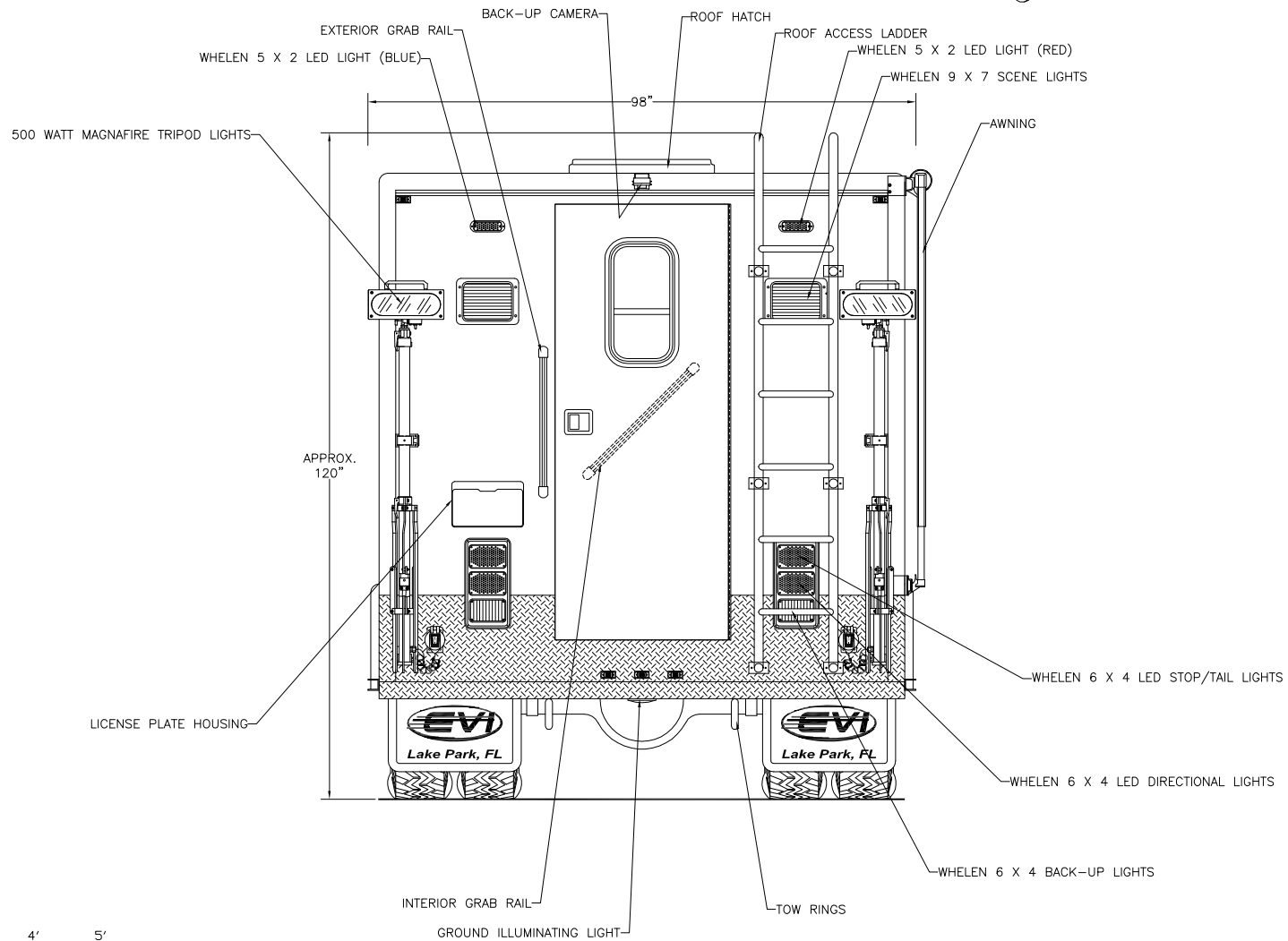
Rear View
