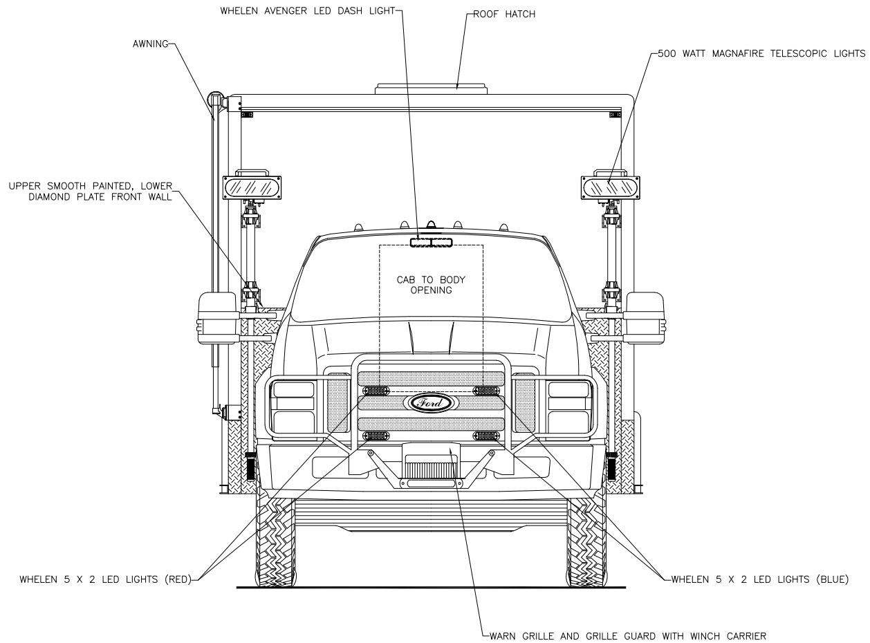
Front View
