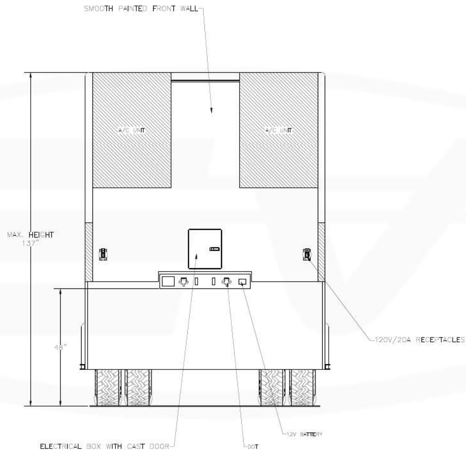
Front View
