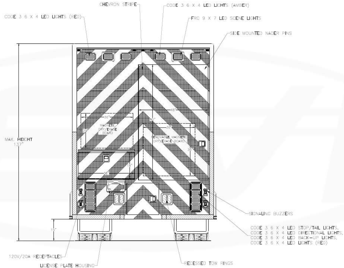
Rear View
