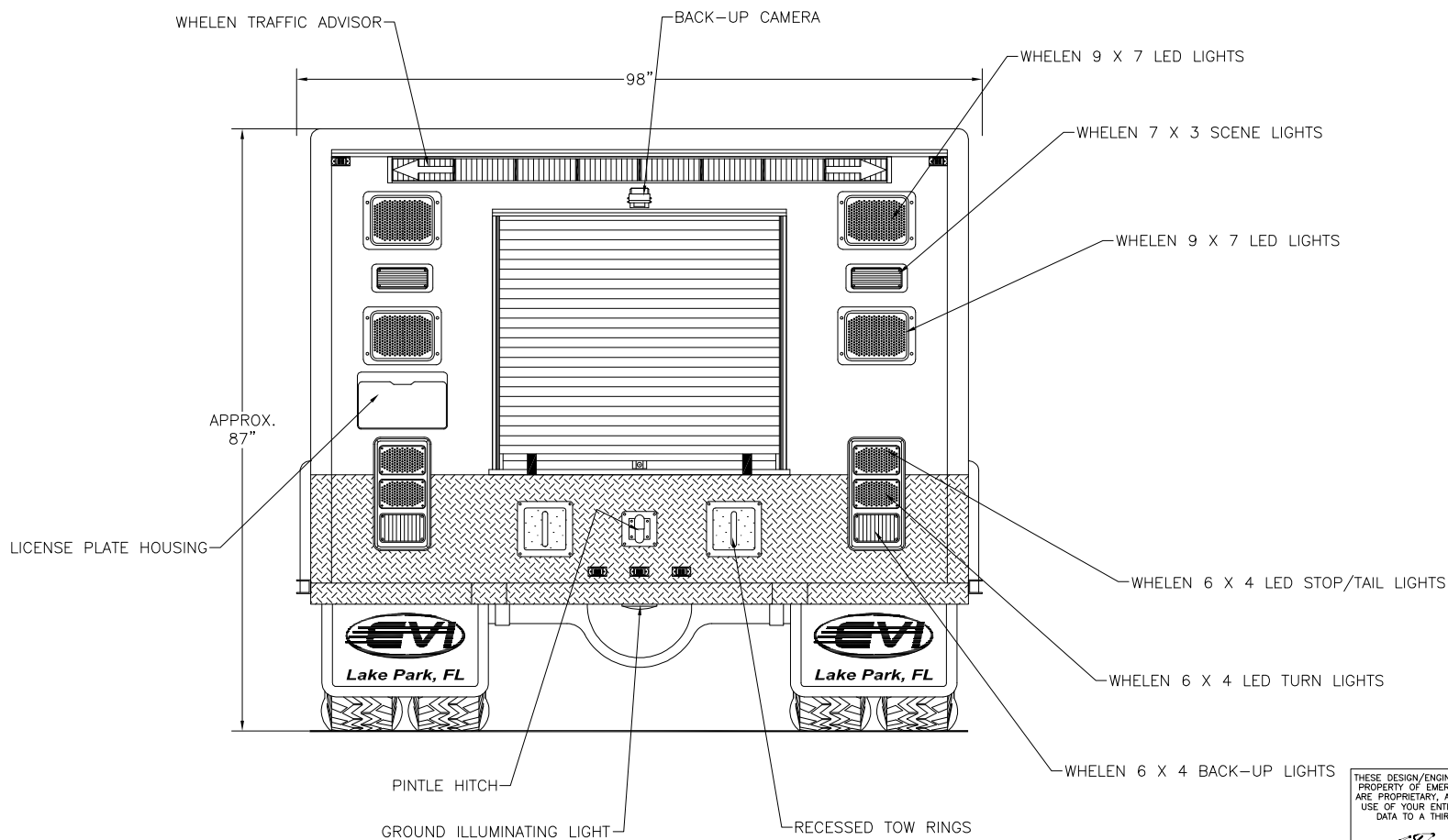
Rear View
