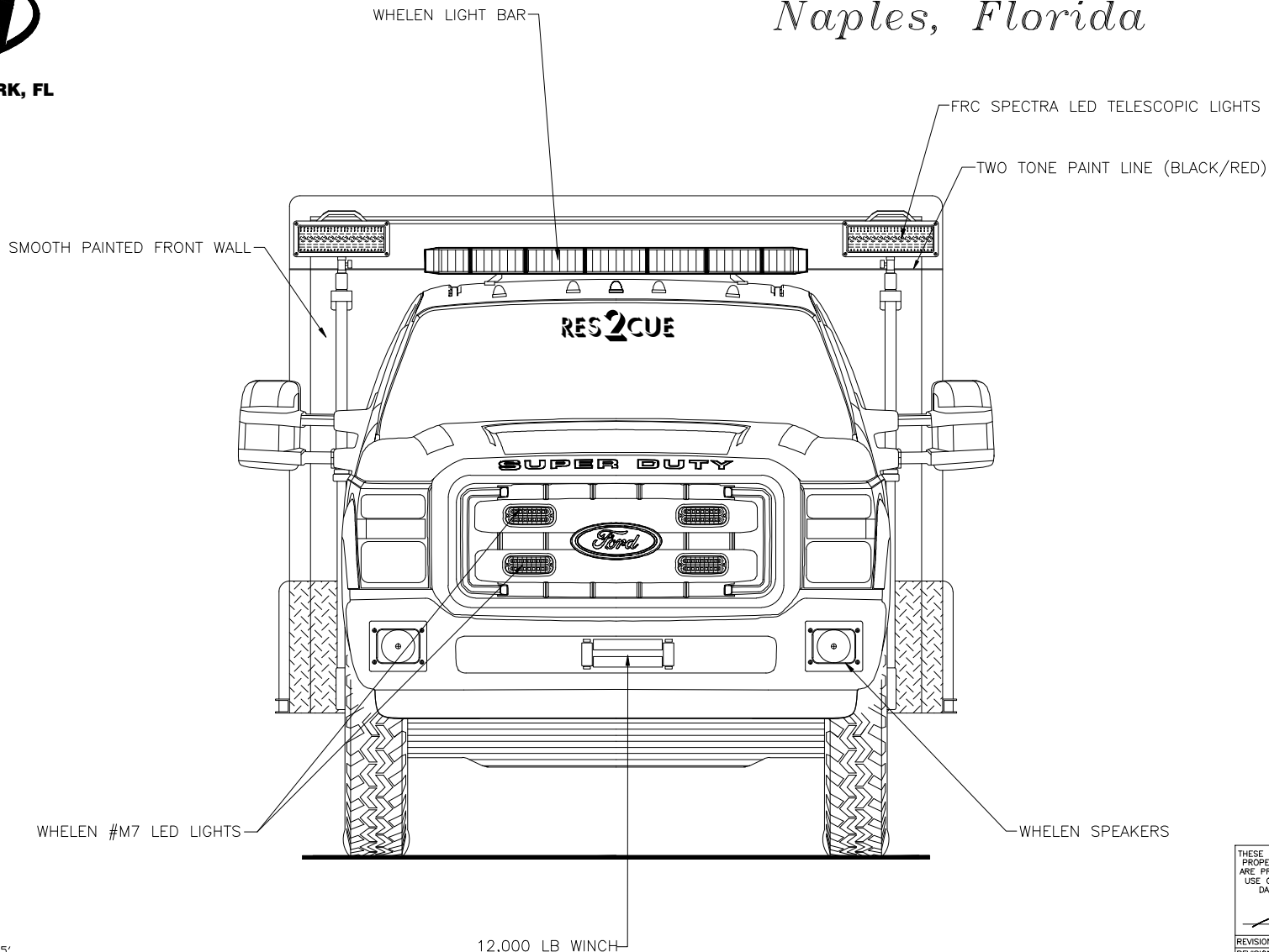
Front View
