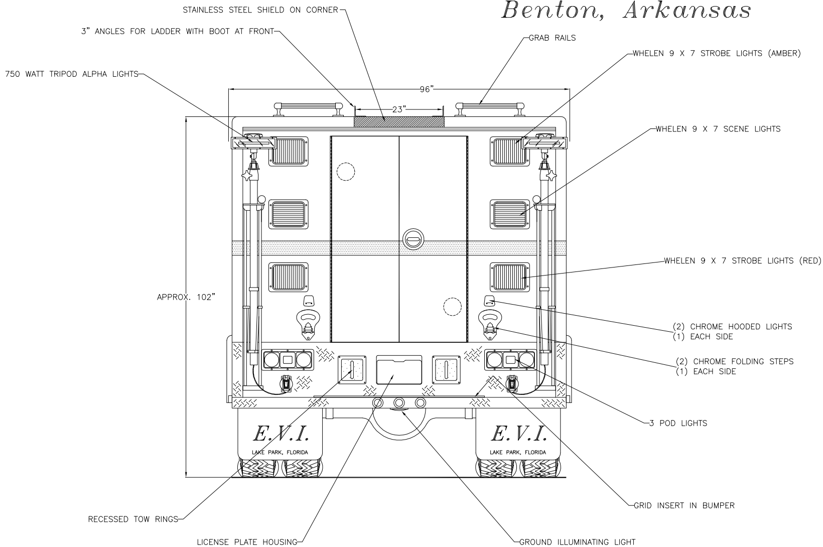
Rear View
