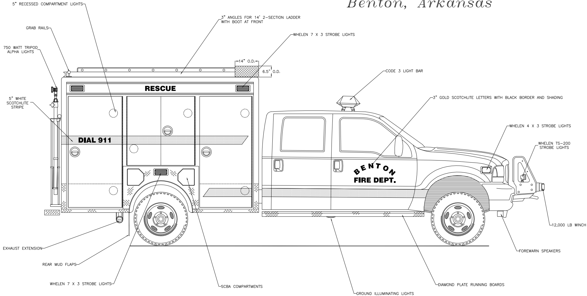
Curbside Overall
