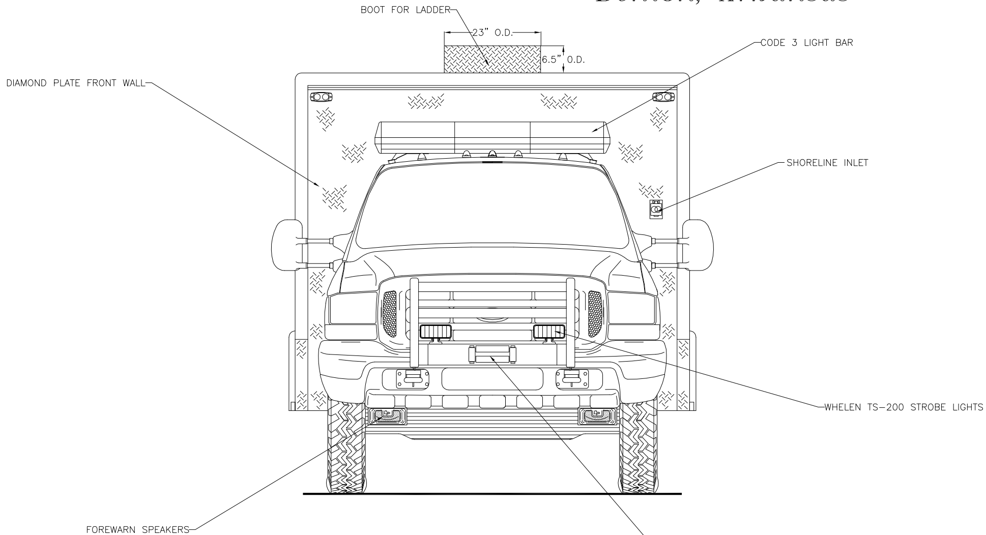
Front View
