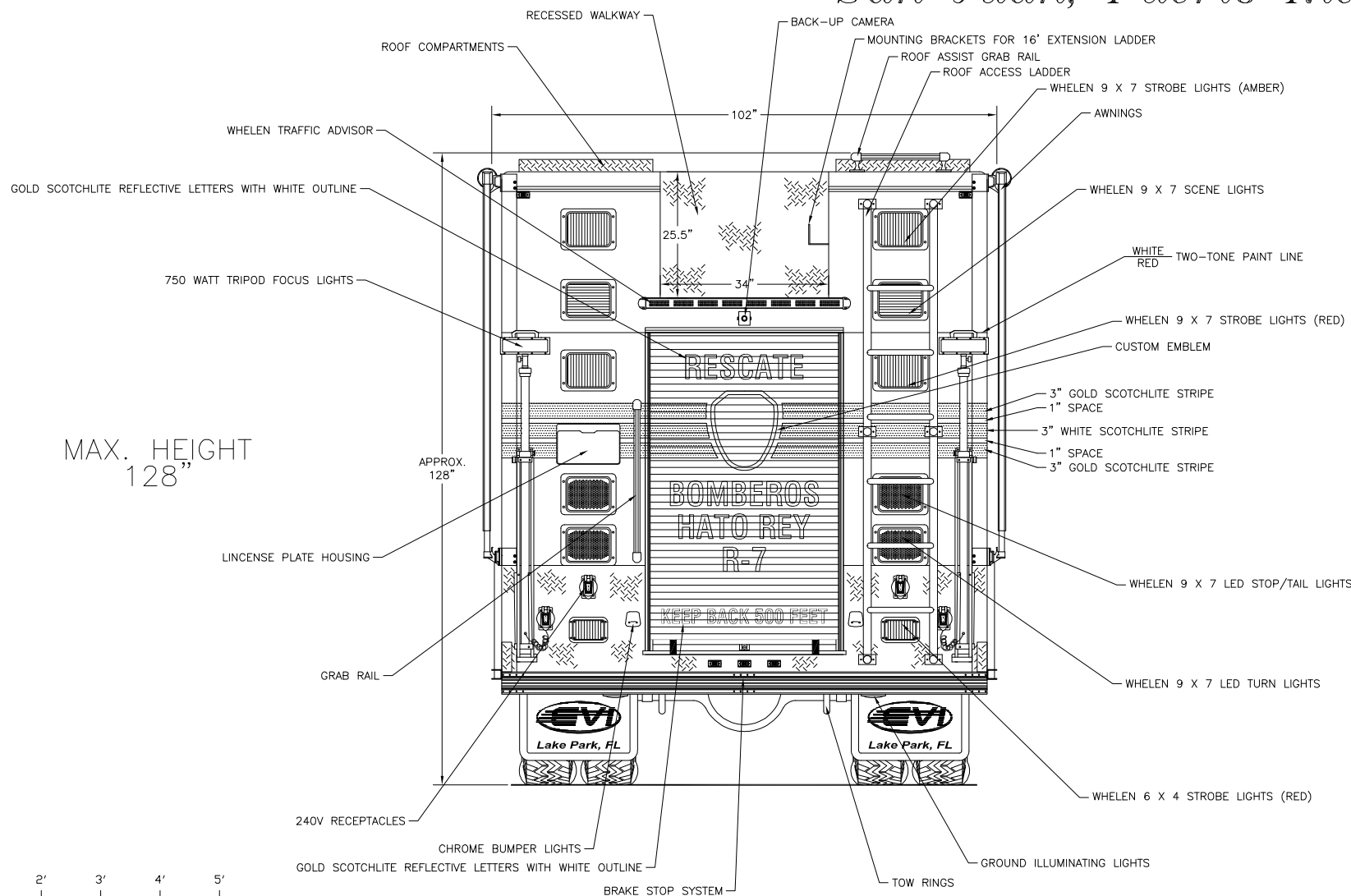
Rear View
