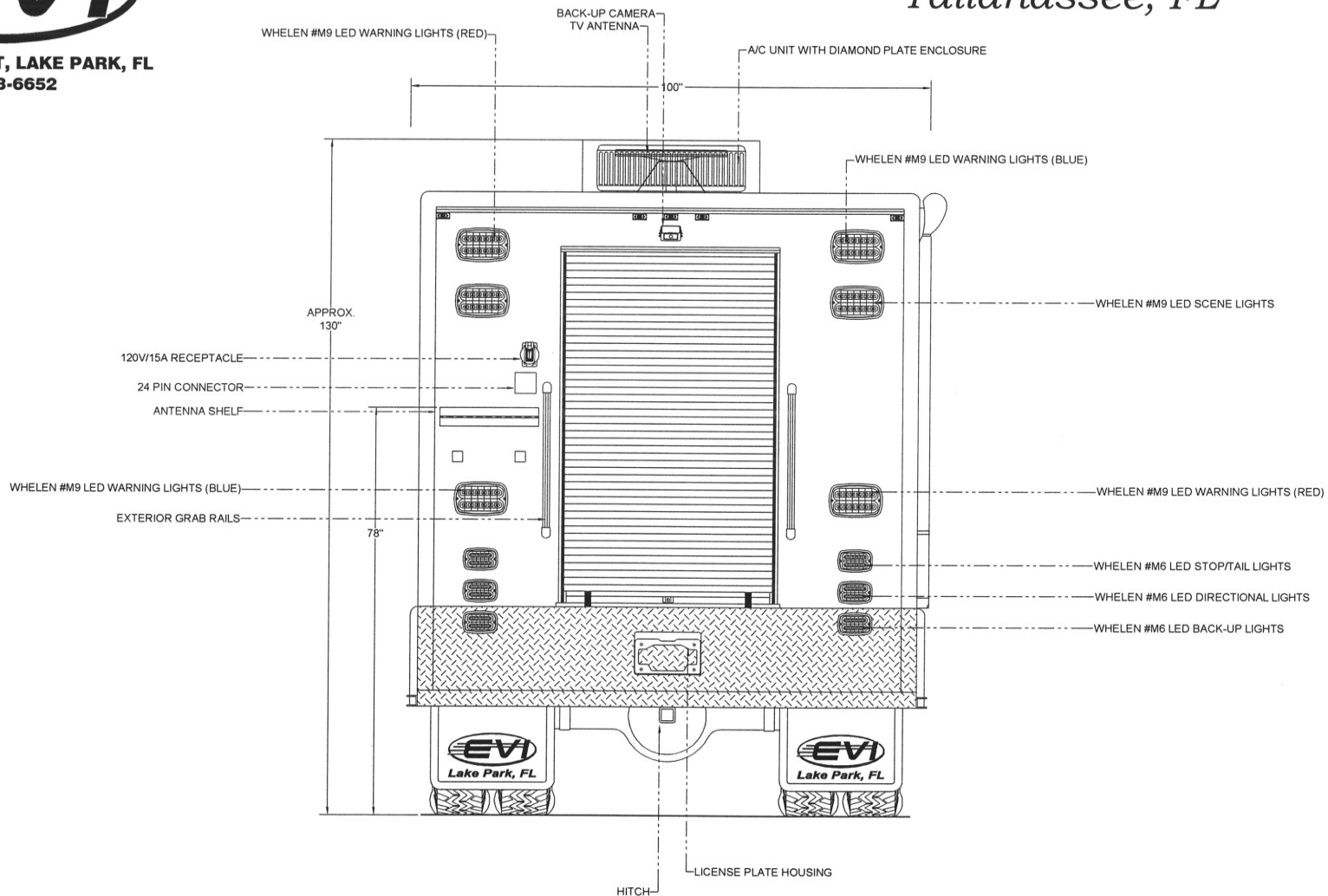
Rear View
