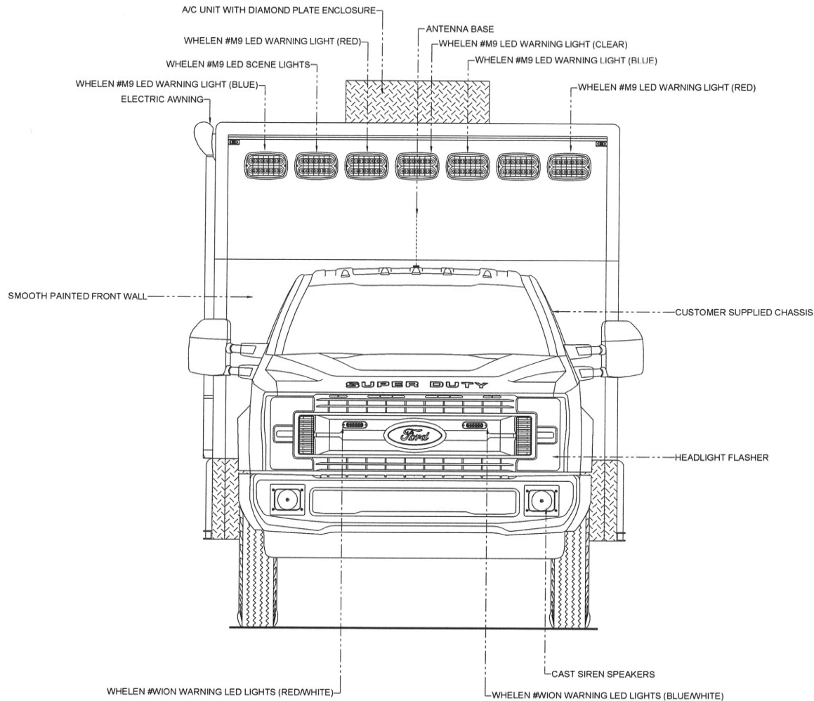
Front View
