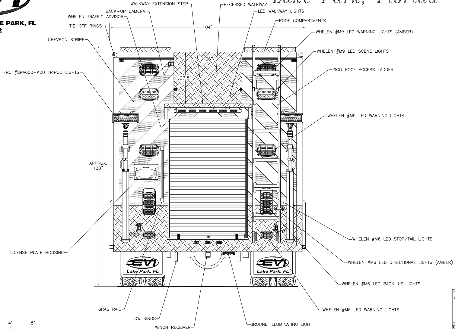
Rear View
