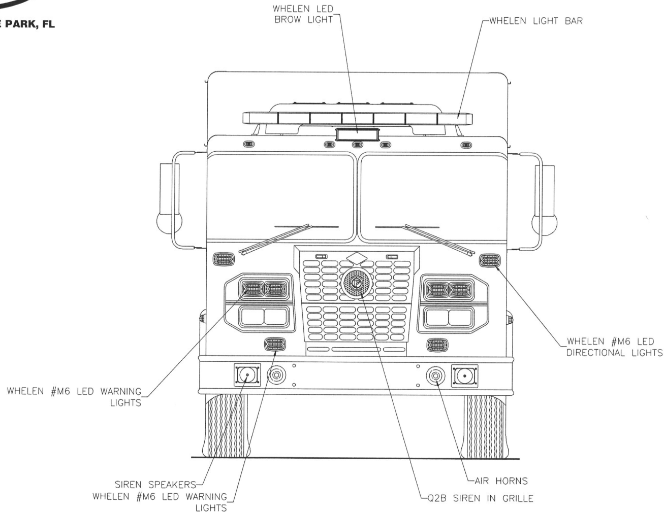
Tractor Front View
